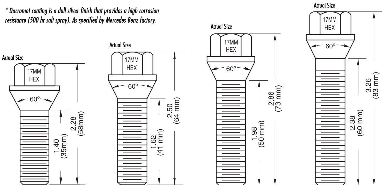
Dacromet 73mm - Overall 50mm - Shank
