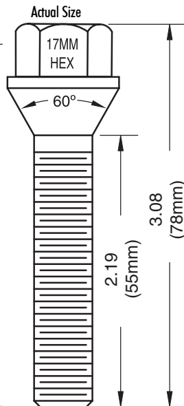
Dacromet 78mm - Overall 55mm - Shank
