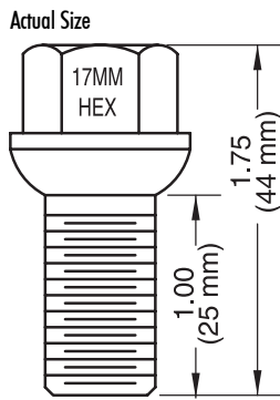
Dacromet 44mm - Overall 25mm - Shank
