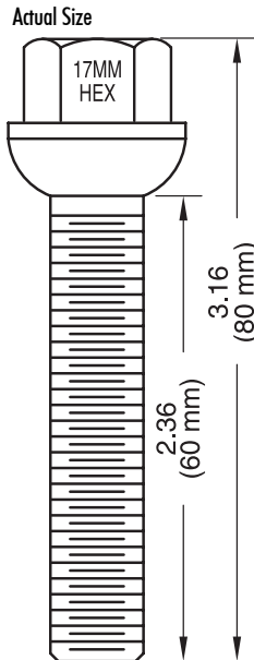
Dacromet 80mm - Overall 60mm - Shank
