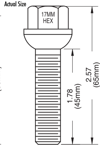
Dacromet 65mm - Overall 45mm - Shank
