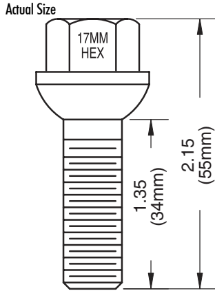
Dacromet 55mm - Overall 34mm - Shank
