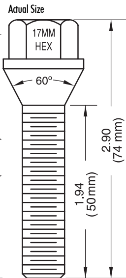
Dacromet 74mm - Overall 50mm - Shank
