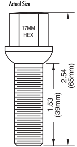
14mm Ball Seat Chromed Lug Bolt 65mm - Overall 39mm - Shank
