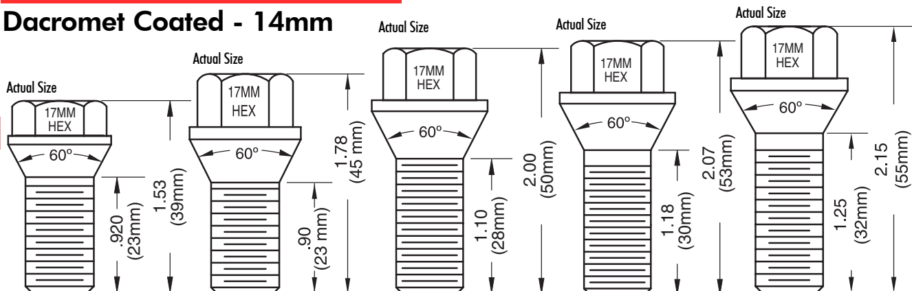
Dacromet 39mm - Overall 23mm - Shank
