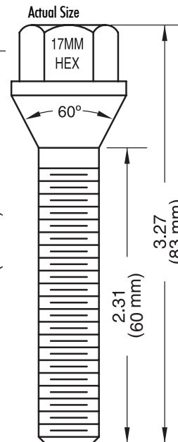
Dacromet 83mm - Overall 60mm - Shank
