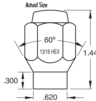
Standard/Chromed 13/16" Hex
