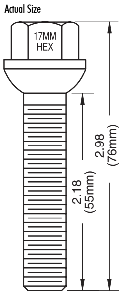
Dacromet 76mm - Overall 55mm - Shank
