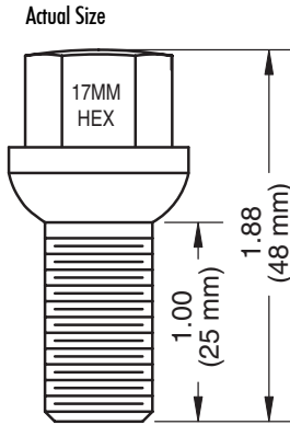
14mm Ball Seat Chromed Lug Bolt 48mm - Overall 25mm - Shank
