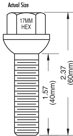
Dacromet 60mm - Overall 40mm - Shank
