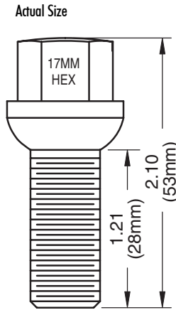
14mm Ball Seat Chromed Lug Bolt 53mm - Overall 28mm - Shank
