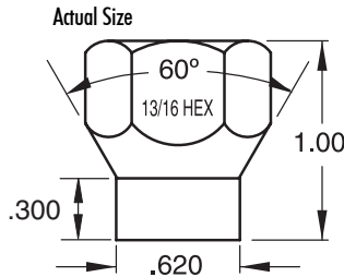
Open End/Chromed 13/16" Hex
