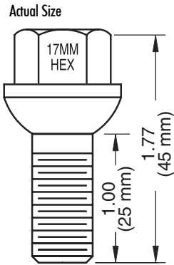
Dacromet 45mm - Overall 25mm - Shank
