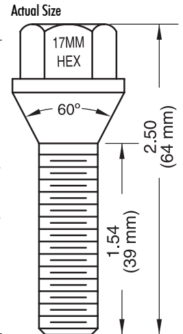
Dacromet 64mm - Overall 39mm - Shank
