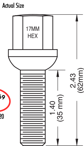
12mm Ball Seat Chromed Lug Bolt 62mm - Overall 35mm - Shank
