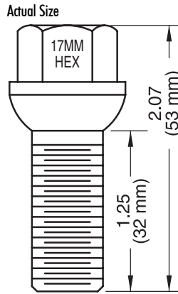
Dacromet 53mm - Overall 32mm - Shank
