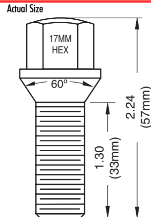
Chrome 57mm - Overall 33mm - Shank
