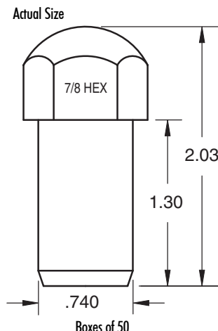
Extra Long/Chromed 7/8" Hex
