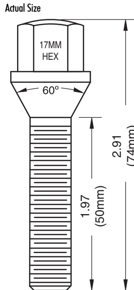
Chrome 74mm - Overall 50mm - Shank
