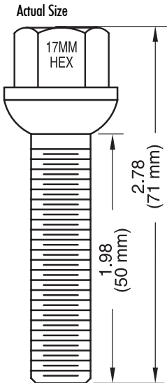
Dacromet 71mm - Overall 50mm - Shank
