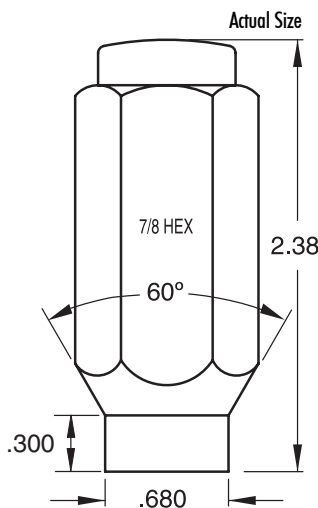
Extra Long/Chromed 7/8" Hex
