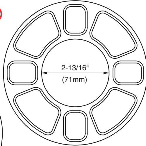
Spacer drawing not to scale
