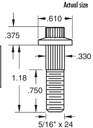
Chrome Plated 12pt Stainless Steel Bolt
