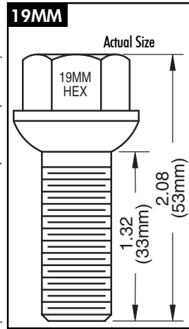
Dacromet 53mm - Overall 33mm - Shank
