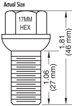
Dacromet 46 mm - Overall 27 mm - Shank
