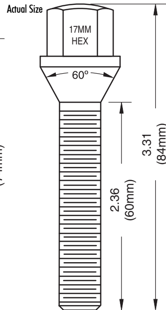
Chrome 84mm - Overall 60mm - Shank
