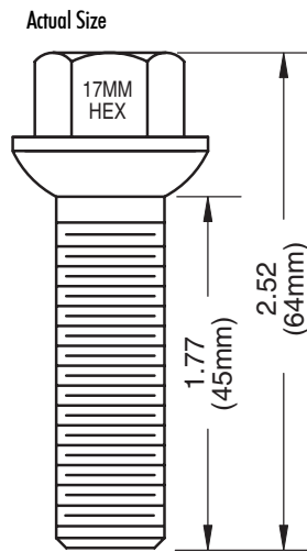
Dacromet 64mm - Overall 45mm - Shank
