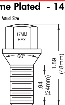
Chrome 48mm - Overall 24mm - Shank
