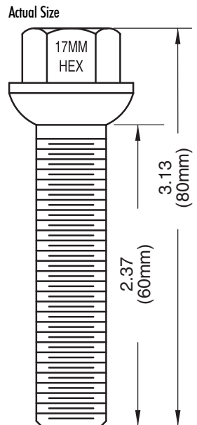
Dacromet 80mm - Overall 60mm - Shank
