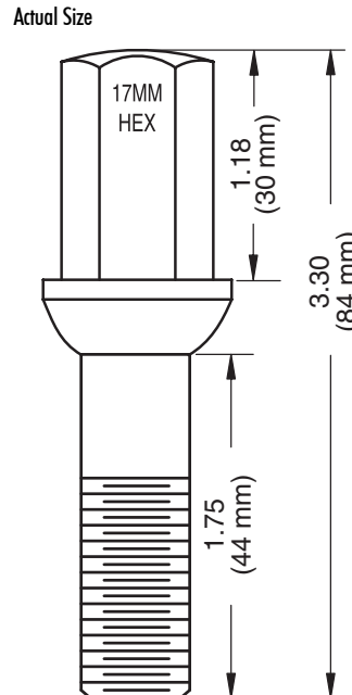
14mm Ball Seat 140 Series Chromed Lug Bolt Normally used on factory Mercedes alloy wheels 84mm - Overall 44mm - Shank
