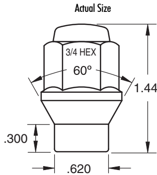
Bulge Style/Chromed 3/4" Hex
