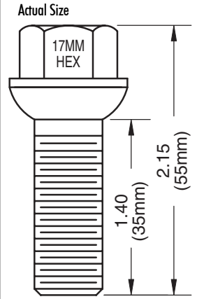
Dacromet 55mm - Overall 35mm - Shank
