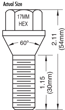
Dacromet 54mm - Overall 30mm - Shank
