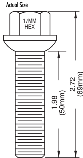
Dacromet 69mm - Overall 50mm - Shank
