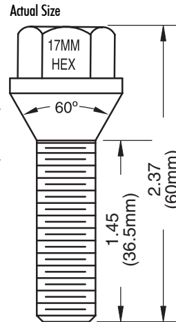
Dacromet 60mm - Overall 36.5mm - Shank
