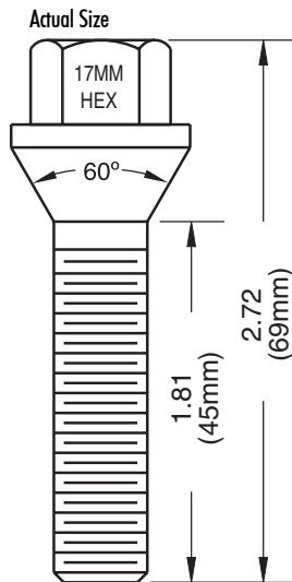
Dacromet 69mm - Overall 45mm - Shank
