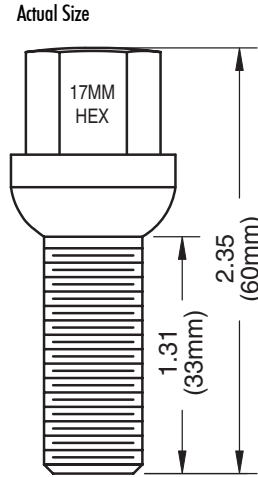
14mm Ball Seat Chromed Lug Bolt 60mm - Overall 33mm - Shank
