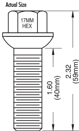
Dacromet 59mm - Overall 40mm - Shank
