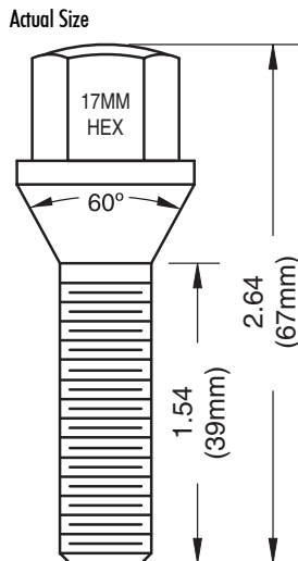
Chrome 67mm - Overall 39mm - Shank
