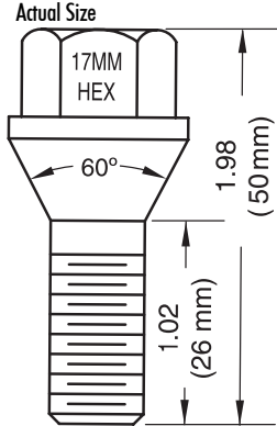
Dacromet 50mm - Overall 26mm - Shank
