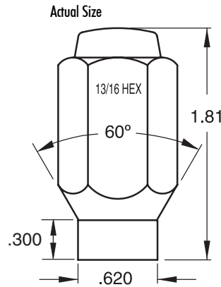
Long/Chromed 13/16" Hex
