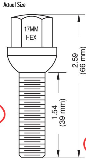
Medium Ball Seat 190/300 Chromed Lug Bolt Normally used on late, flat faced style factory Mercedes alloy wheels
