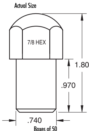
Standard/Chromed 7/8" Hex
