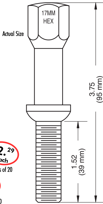
Extra Long Ball Seat 560 Chromed Lug Bolt Normally used on late, 560 series flat faced style factory Mercedes alloy wheels
