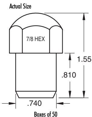
Short/Chromed 7/8" Hex
