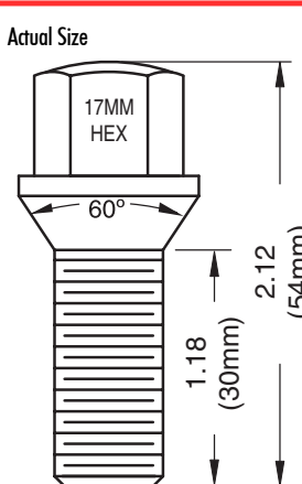
Chrome 54mm - Overall 30mm - Shank
