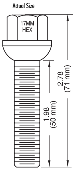
SL Spacer Chromed Lug Bolt Normally used with our SL spacer see page #36
