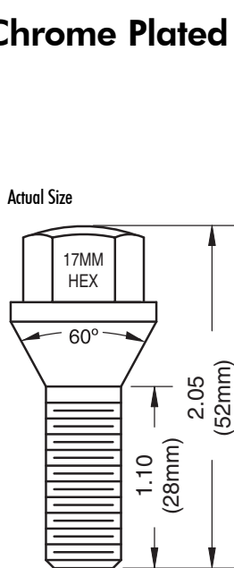
Chrome 52mm - Overall 28mm - Shank
