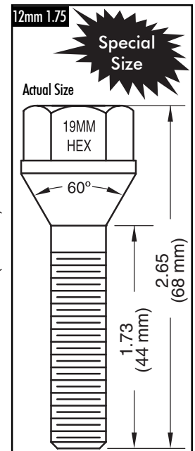
Dacromet 68mm - Overall 44mm - Shank
