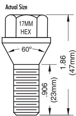
Dacromet 47mm - Overall 23mm - Shank
