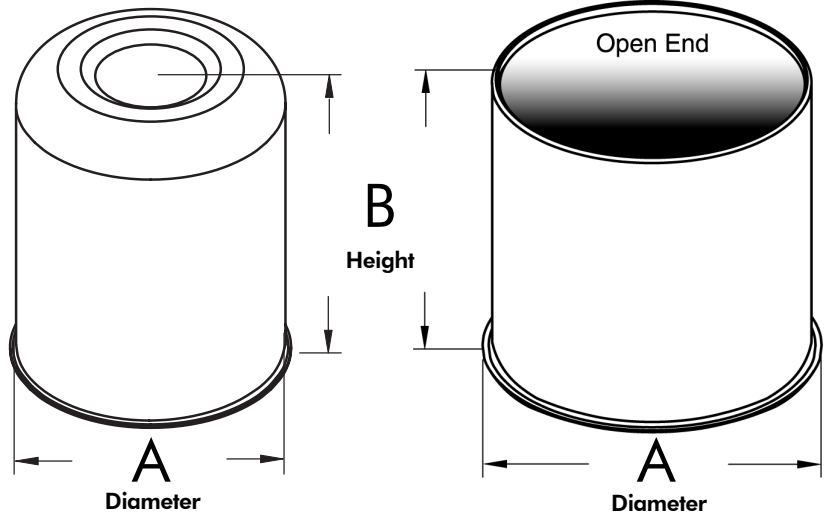
Open End Drawing not to scale
