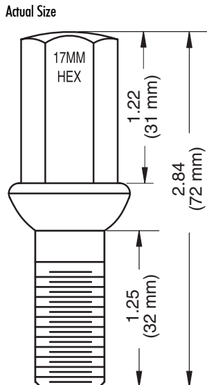
14mm Ball Seat 140 Series Chromed Lug Bolt Normally used on aftermarket Mercedes alloy wheels 72mm - Overall 32mm - Shank
