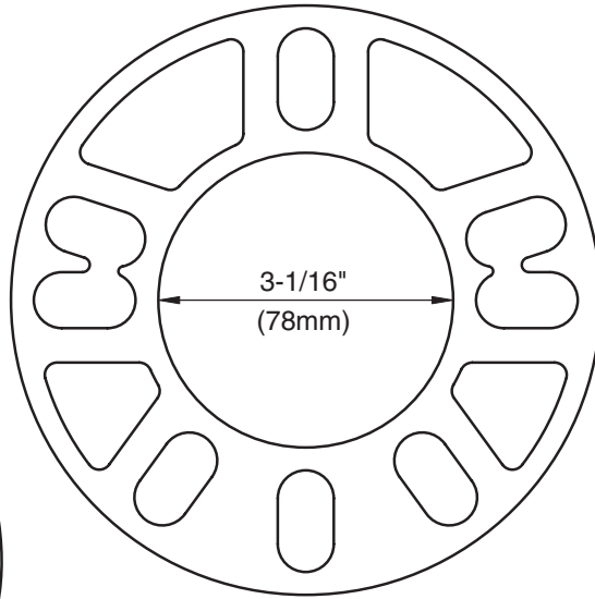
Spacer drawing not to scale
