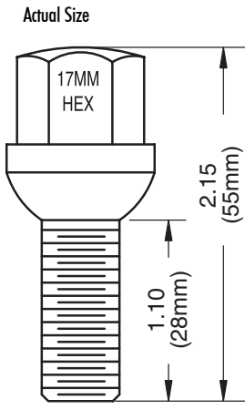
Short Ball Seat Early Chromed Lug Bolt Normally used on early factory Mercedes 14" alloy wheels up thru 1985 models
